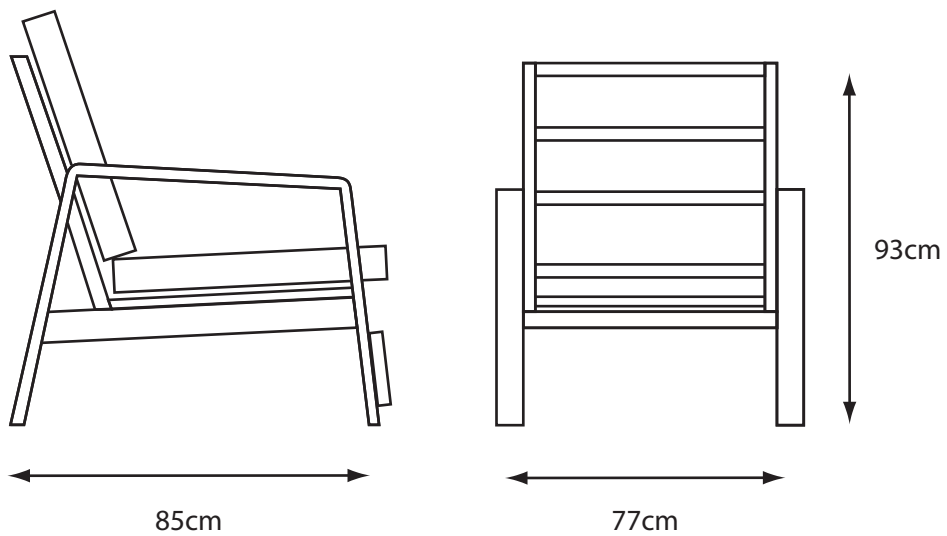
Barcelona 4 Seat Reclining Set
